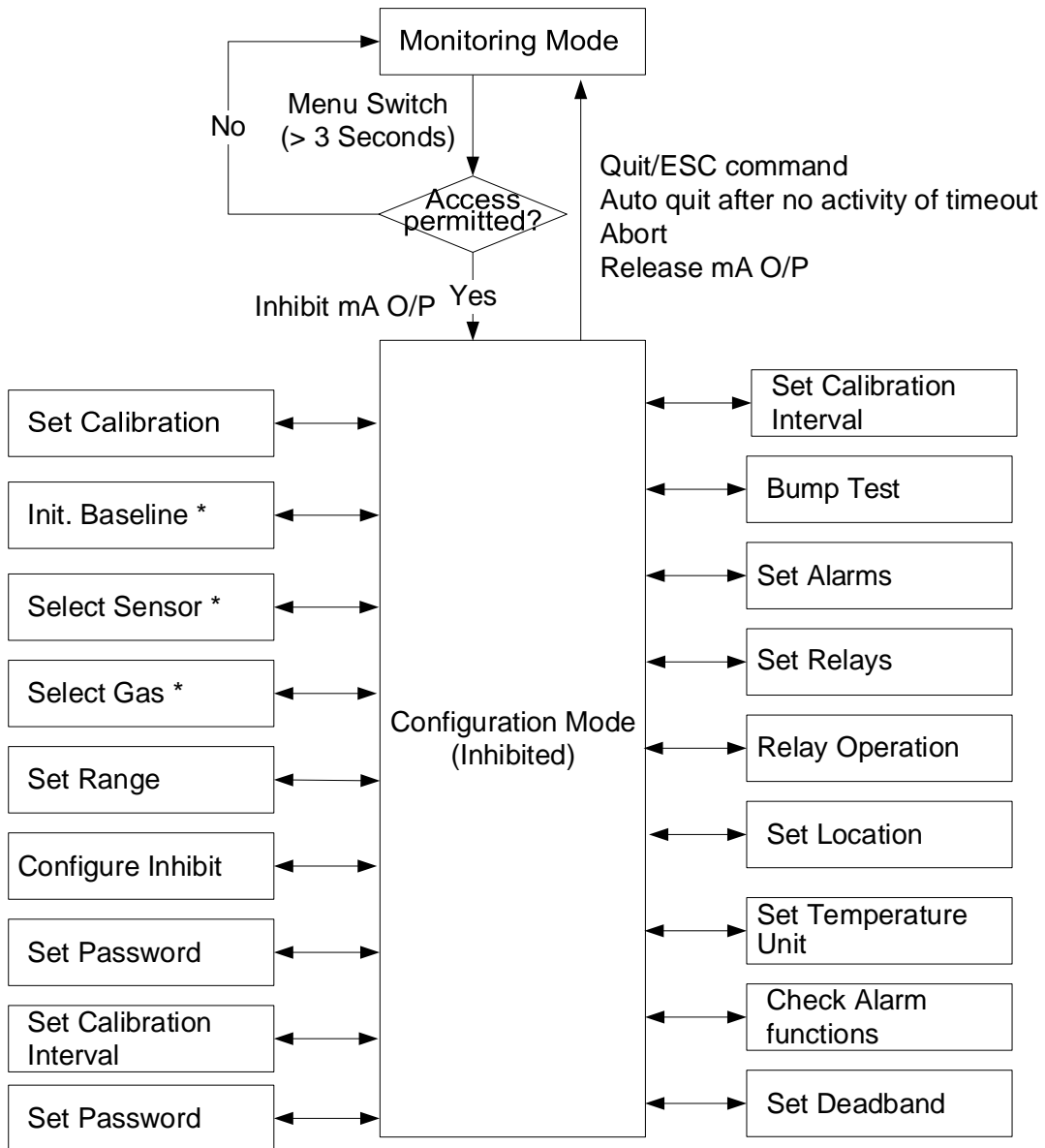
Diagram 17 Configuration Mode
