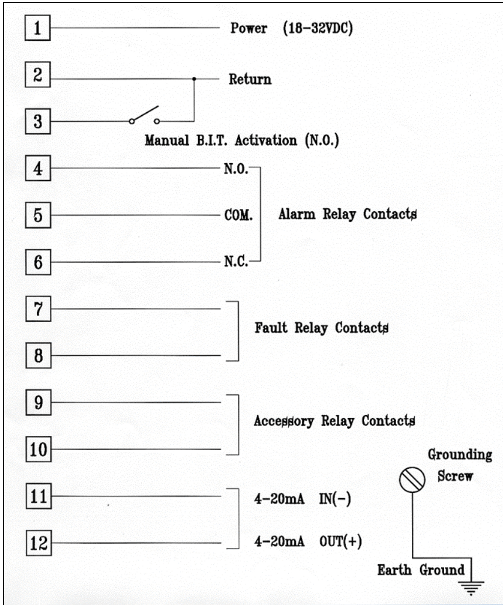
Figure 7. Flame Detector Assembly - Wiring Diagram
