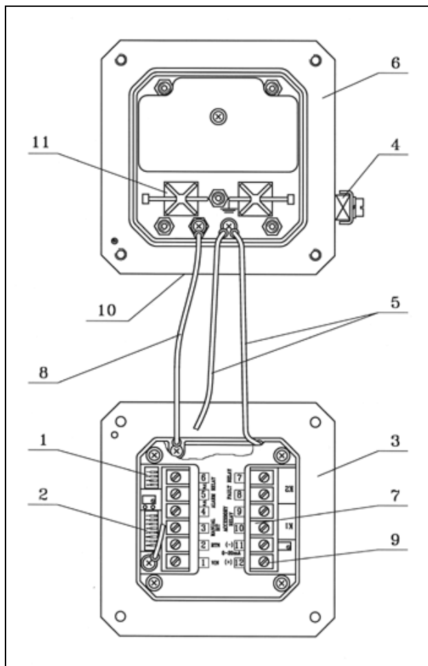
Figure 5. UV/IR Flame Detector with Cover Removed
