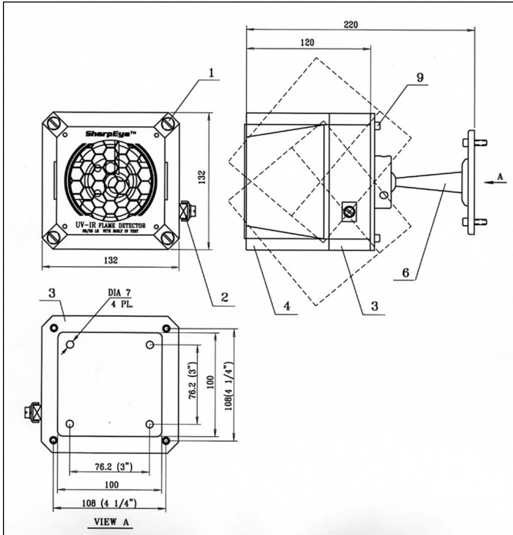
Figure 4.a. U/IR Detector and Swivel Mount Assembly
