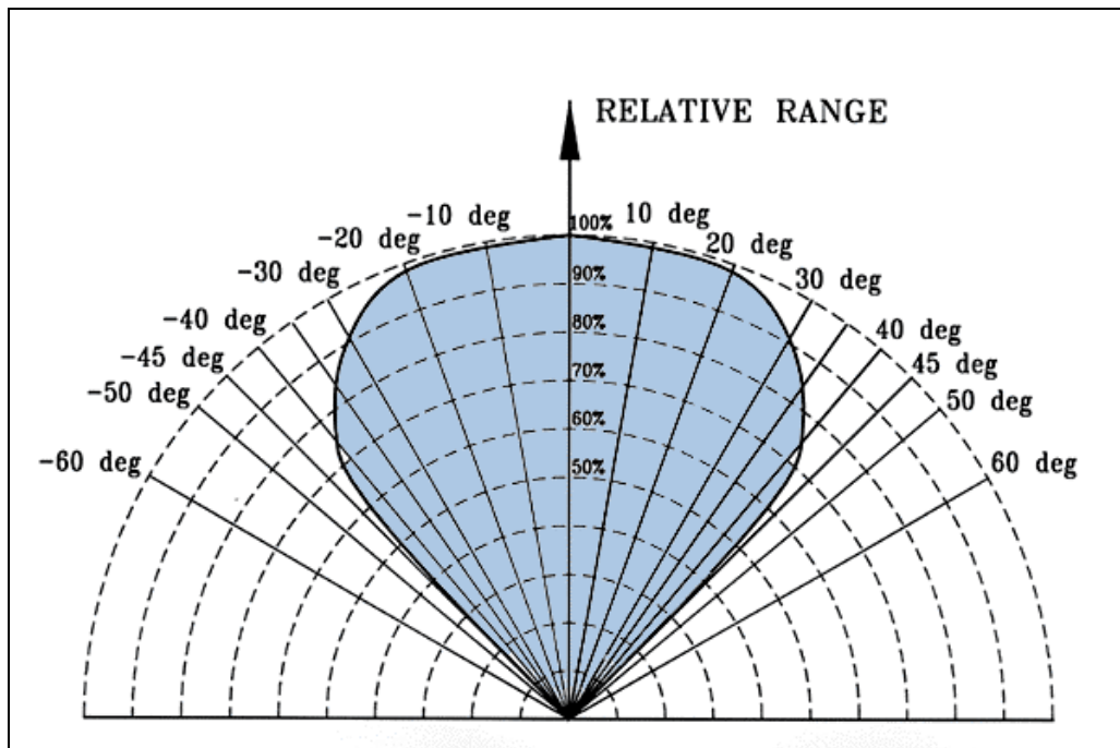
Figure 3. Horizontal and Vertical Fields of View
