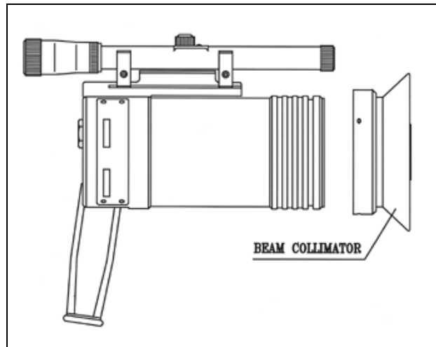
Figure 13: Fire Simulator
