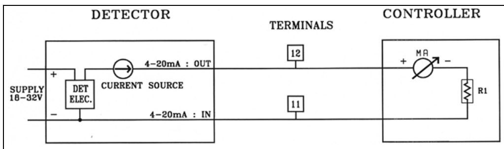
Figure 9. Wiring Diagram for 4-20mA
