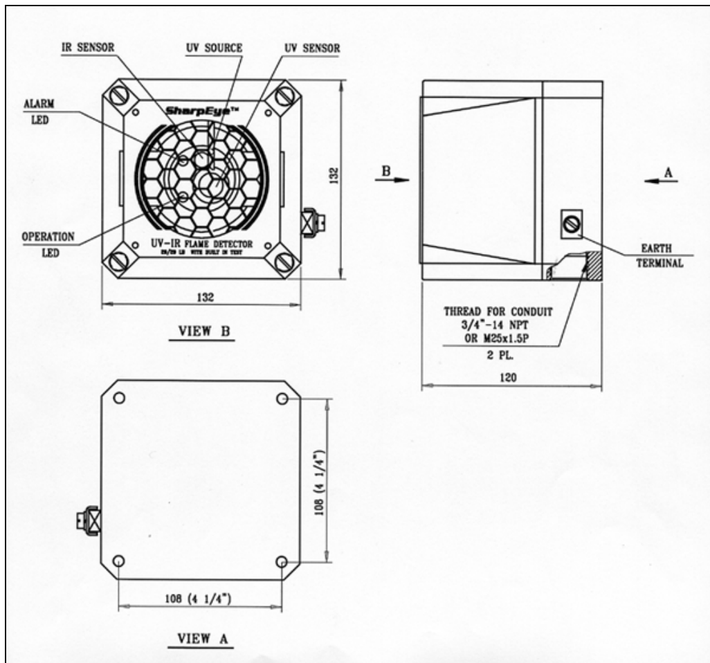
Figure 1. Flame Detector Assembly - Outline Drawing
