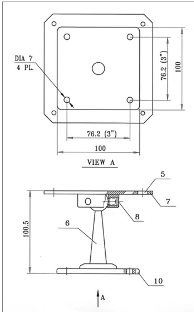
Figure 4.b. Swivel Mount Assembly
