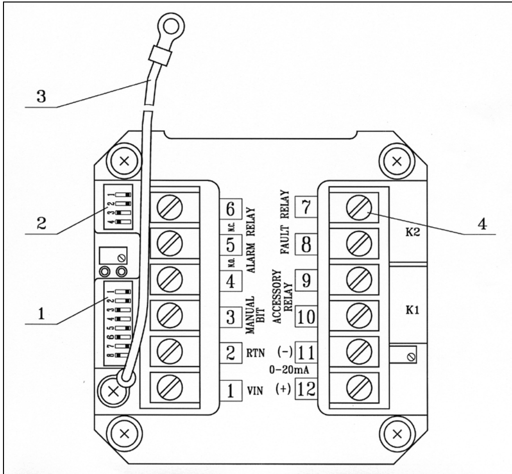
Figure 6. Terminal Board Configuration
