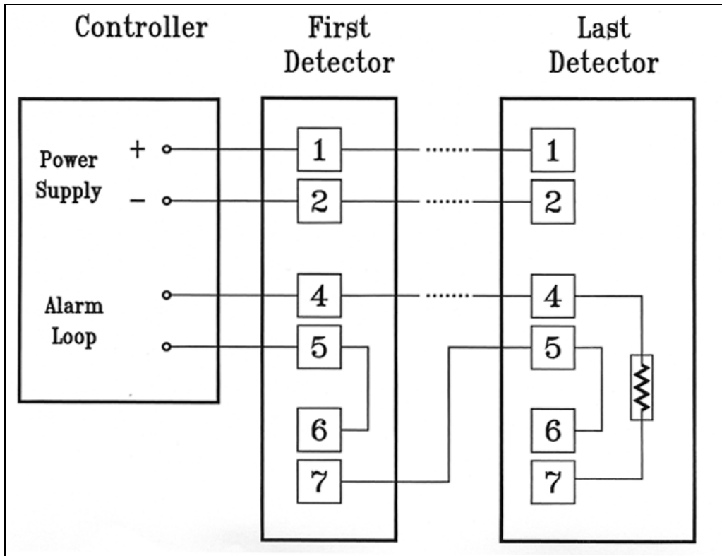
Figure 8. Typical Wiring Diagram for Four-Wire Controller
