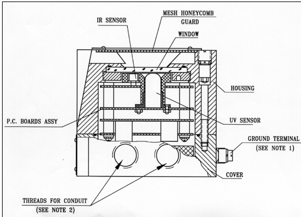
Figure 2. Flame Detector Assembly - Schematic Section
