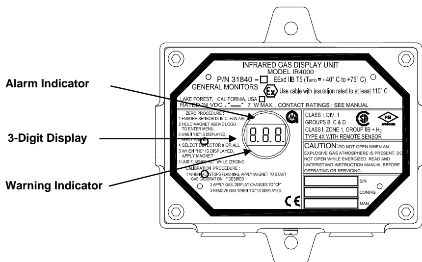
Figure 11: Front Panel Display and Indicators
