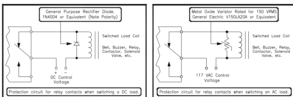
Figure 10: Relay Protection for DC and AC Loads
