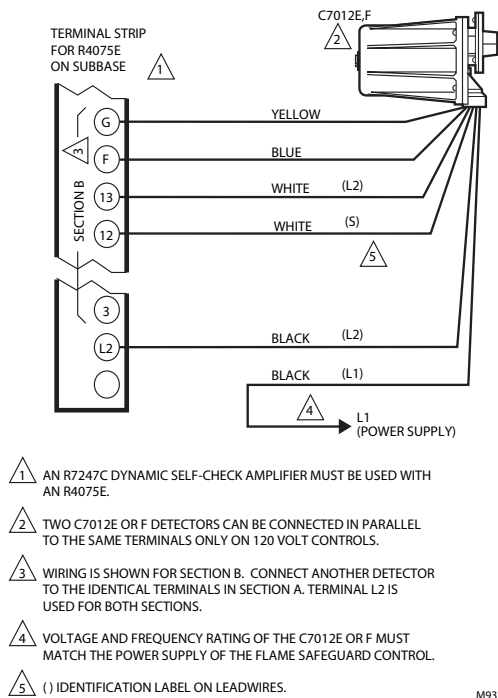
Fig. 12. Wiring diagram for C7012E or F Detectors with R4075E (currently obsolete) Flame Safeguard Control.
