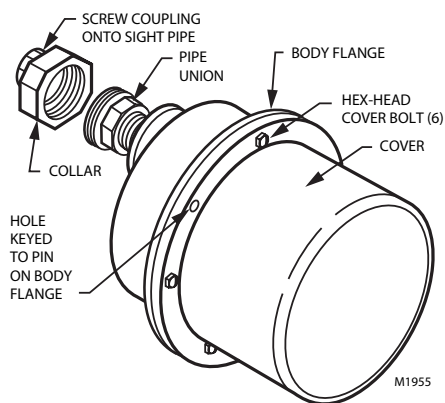
Fig. 8. Mounting C7012C or F Detector.
