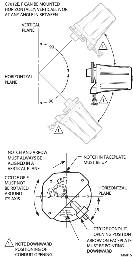
Fig. 6. C7012E,F mounting positions.
