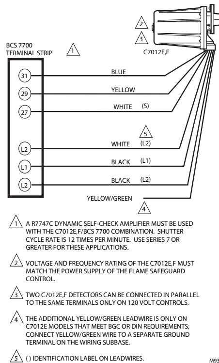
Fig. 15. Wiring diagram for C7012E,F Detectors with BCS 7700 (currently obsolete) Flame Safeguard controls.
