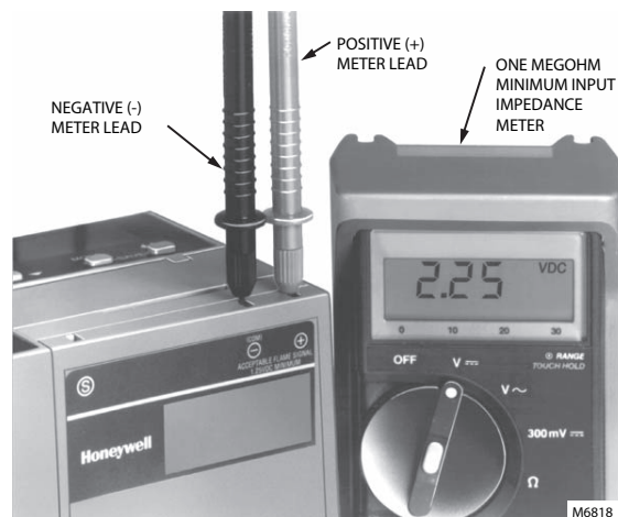
Fig. 20. Measuring voltage flame signal with 7800 Series controls.
