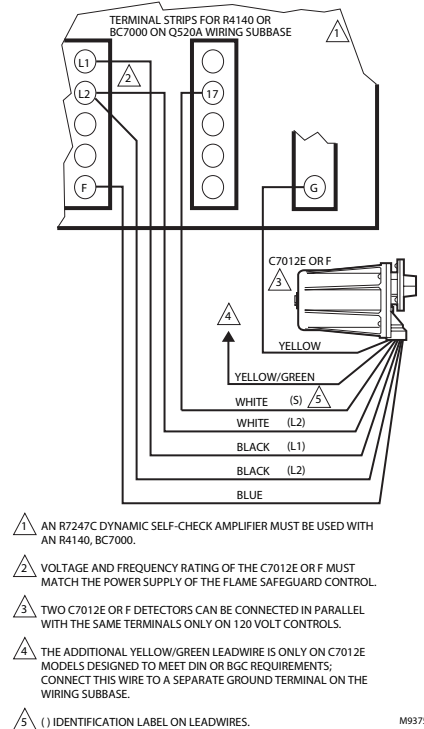
Fig. 14. Wiring diagram for C7012E or F Detectors with R4140, and BC7000 (currently obsolete), and R7140 Flame Safeguard controls.
